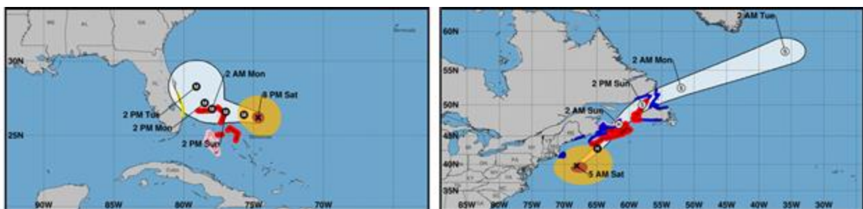
Figure 31: Official 3-day forecasts for Hurricane Dorian showing a large acceleration.
