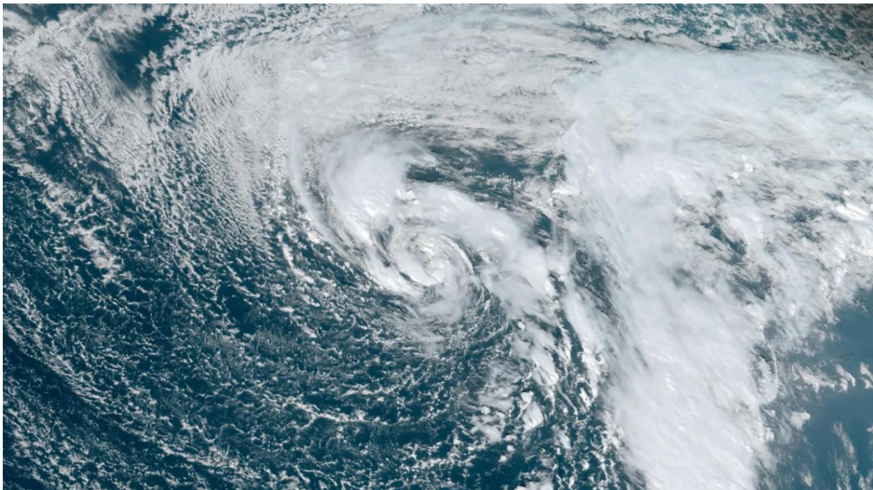
Figure 6: Subtropical Storm Wanda after transitioning from a Nor'easter in 2021.
