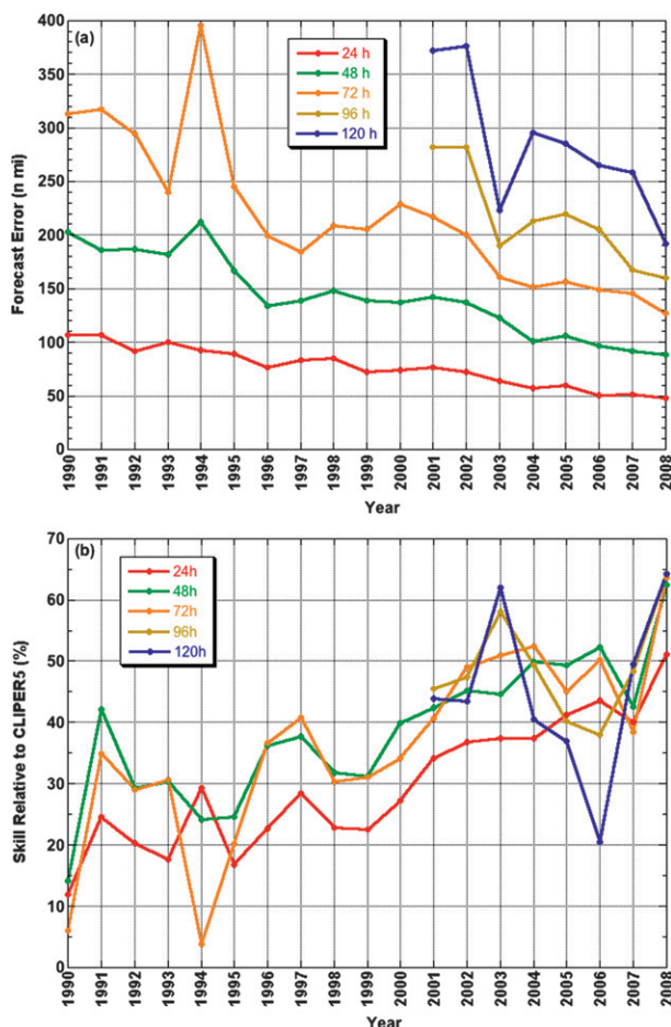
FIG. 4. Recent trends in NHC official track (a) forecast error and (b) skill for the Atlantic basin (all tropical cyclones).
