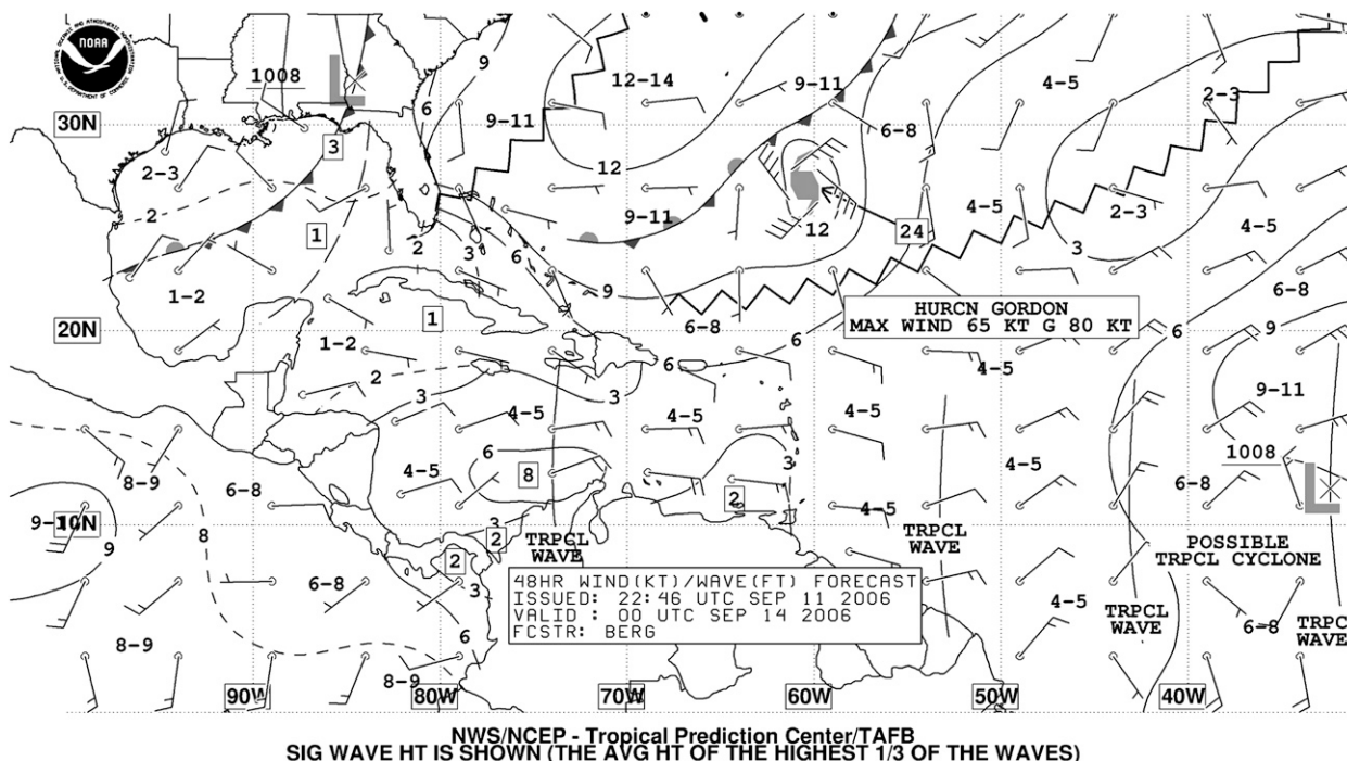
FIG. 2. Atlantic 48-h wind-wave forecast valid at 0000 UTC 14 Sep 2006.
